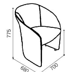
SS.038.2.R - Armchair with castors
